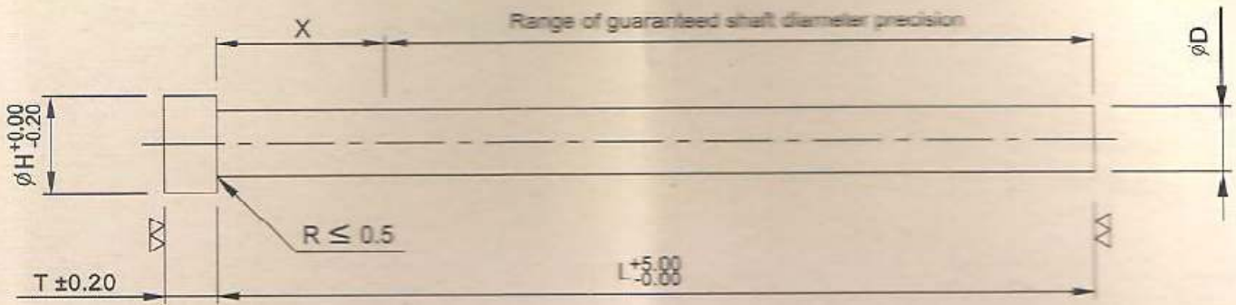
D dimension tolerances
